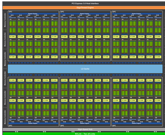
Fig. 12.4.8: NVIDIA Turing architecture (image courtesy of NVIDIA)
